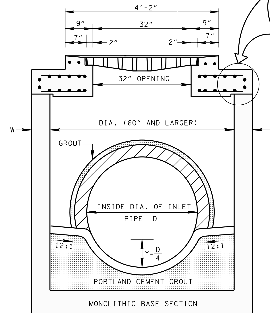
SECTION B-B
